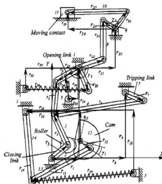
Fig. 1 : Gas insulated circuit breaker
