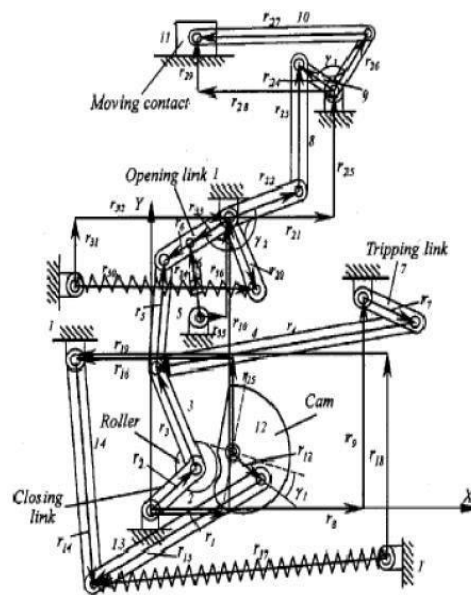
Fig. 2 : Vector loop diagram
