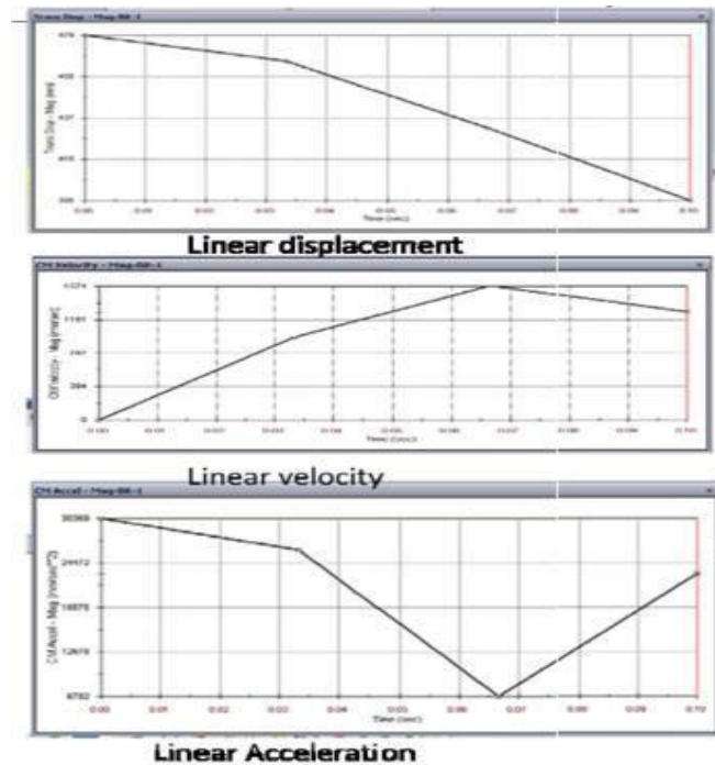
Fig. 7 : Open operation of Link 11
