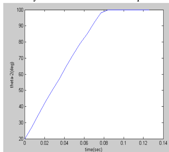
Fig. 4: Follower angular displacement Opening:
