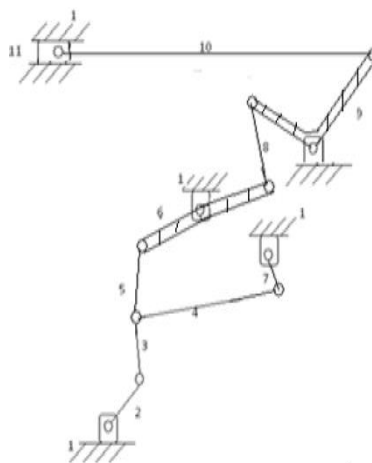
Fig. 3 : Schematic of switch gear mechanism
