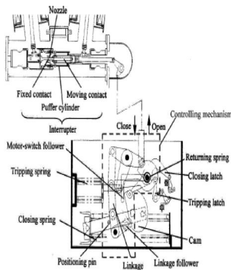
Fig. 1 : Gas insulated circuit breaker
